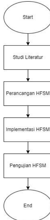
Gambar 1. Flowchart
